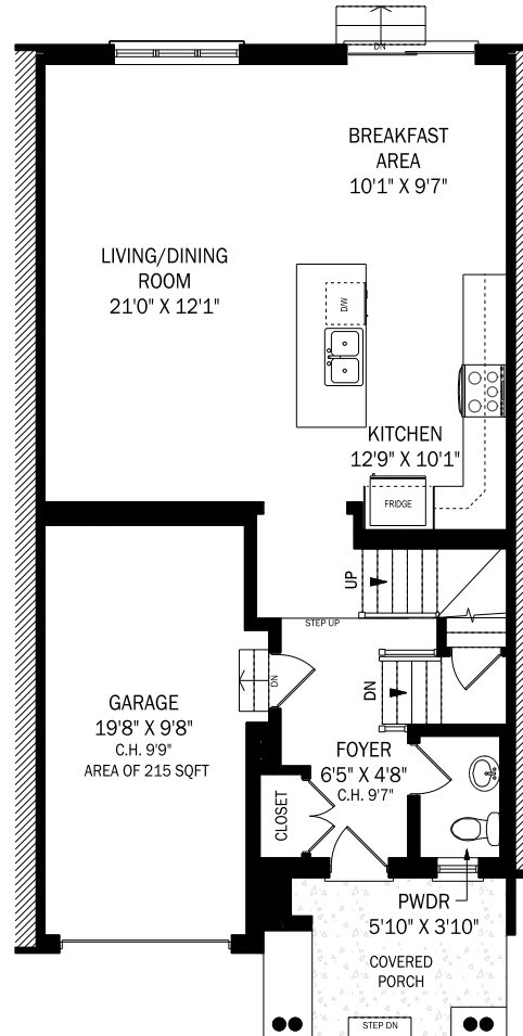
CEILING HEIGHT 9'0" MAIN FLOOR - 745 SQUARE FEET
